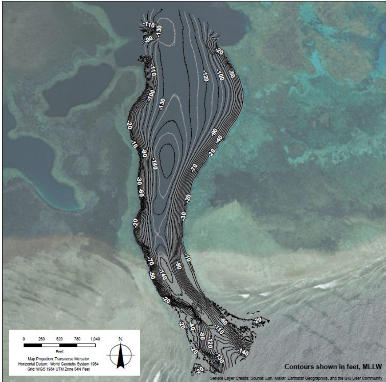
Figure 3-2 Yap Channel Bathymetry (Surveyed May 2023 by Sea Engineering, Inc.)
