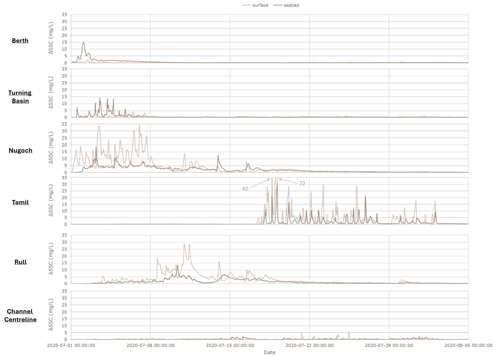
Figure 6-10 Time series \Delta\text{SSC} for each sites during calm scenario
