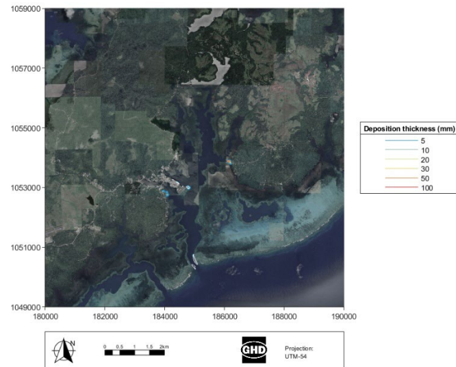
Figure 6-25 The maximum deposition thickness for the windy scenario with site extent (left) and larger domain extent (right) for the Yap Port and surrounds
